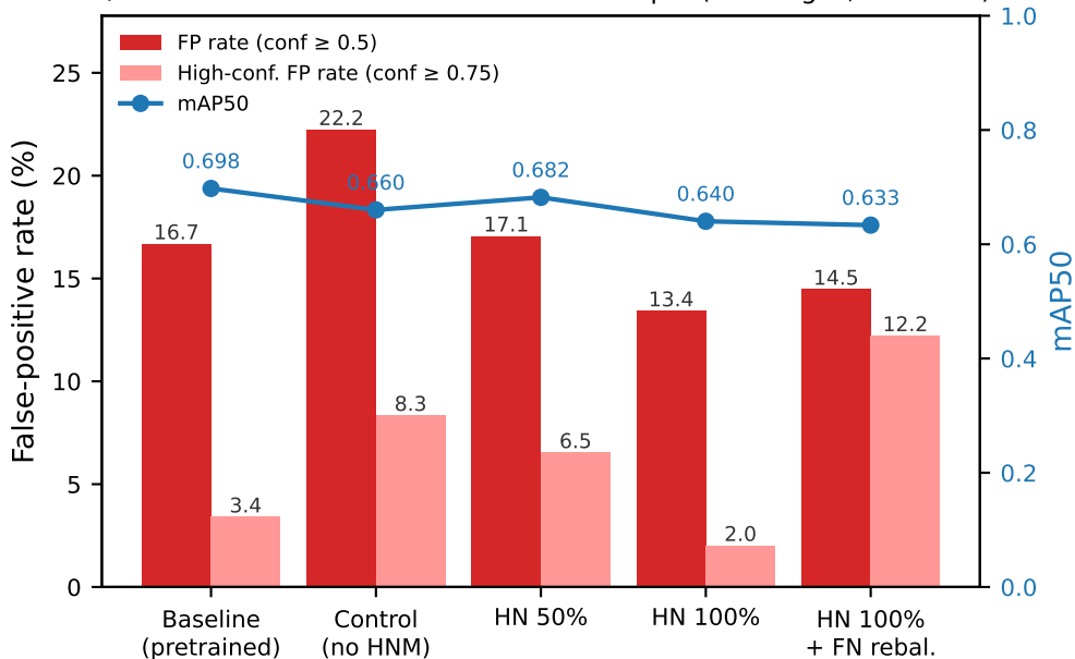
A/B evaluation on the held-out validation split (32 images, seed=42)
