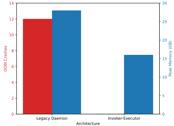
Figure 2: A bar chart comparing OOM crashes and Peak Memory Usage between the Legacy Daemon Setup and the Invoker-Executor Pattern
