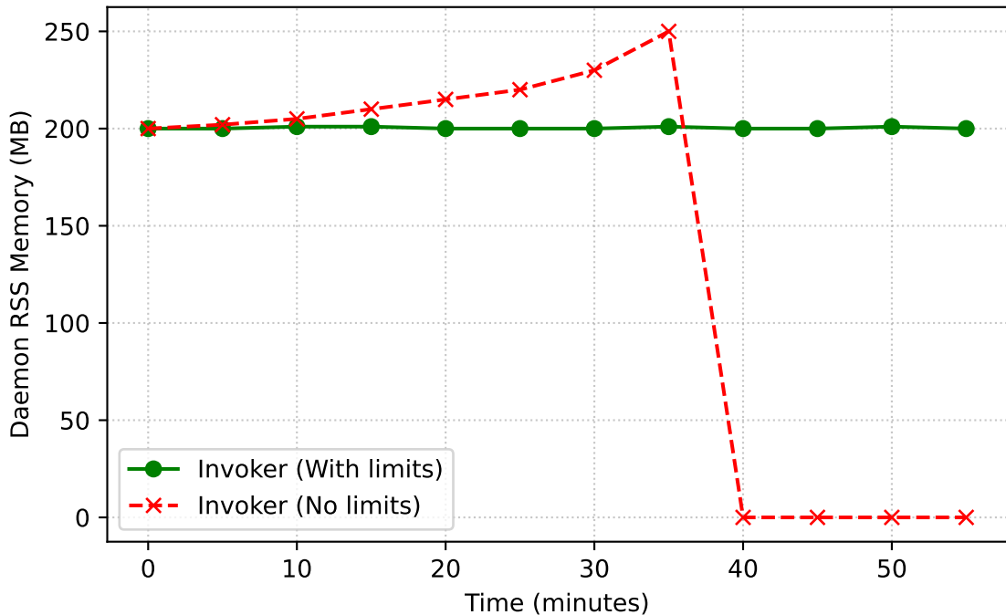
Invoker Memory Stability under YOLO Memory Leaks
