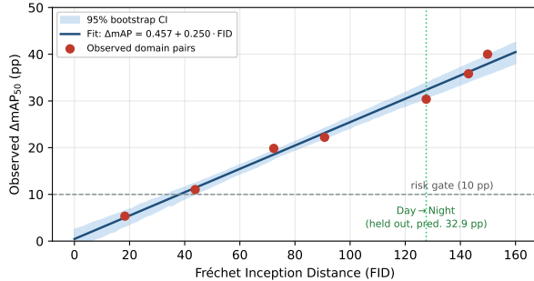
Figure 1: Observed \text{mAP}_{50} degradation versus Fréchet Inception Distance across the seven real domain pairs, with the fitted FID-only predictor and its 95% bootstrap band. The held-out Day \rightarrow Night pair (prediction 32.9 pp, actual 30.4 pp) is highlighted.
