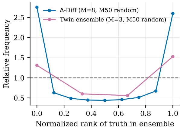
(b) Rank histogram (active pixels)
