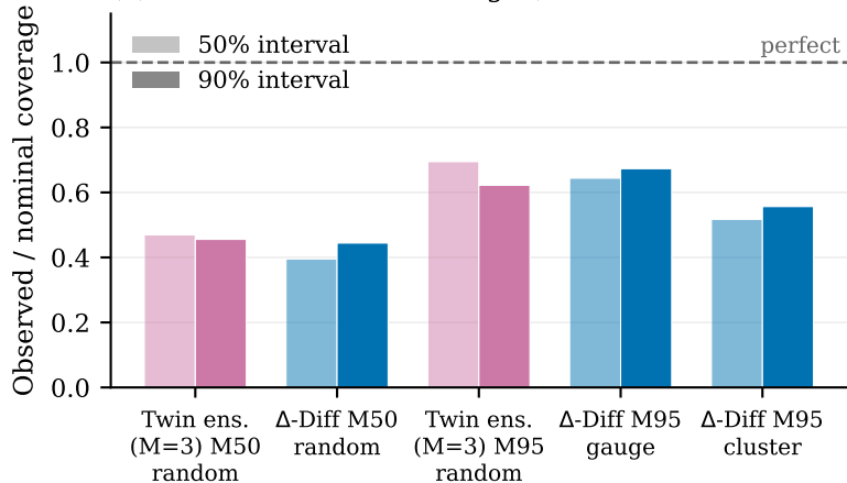
(a) Central-interval coverage (finite-ensemble corrected)
