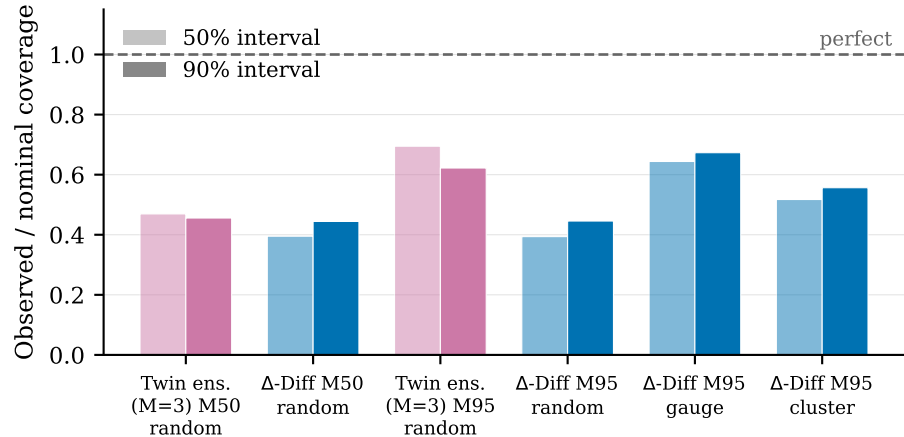
(a) Central-interval coverage (finite-ensemble corrected)
