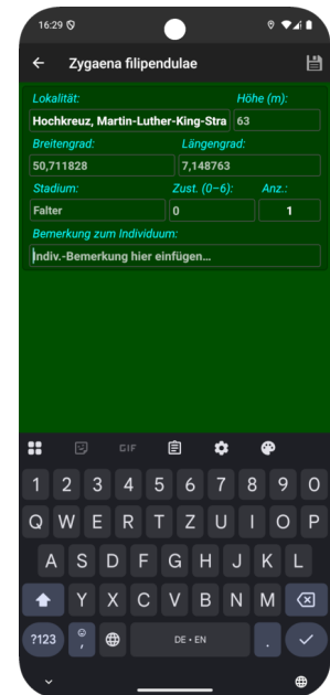
Abb. 6: Individuum editieren
