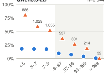
Qwen3.5-2B n=6,944
