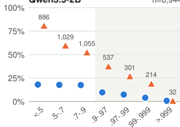
Qwen3.5-2B n=6,944
