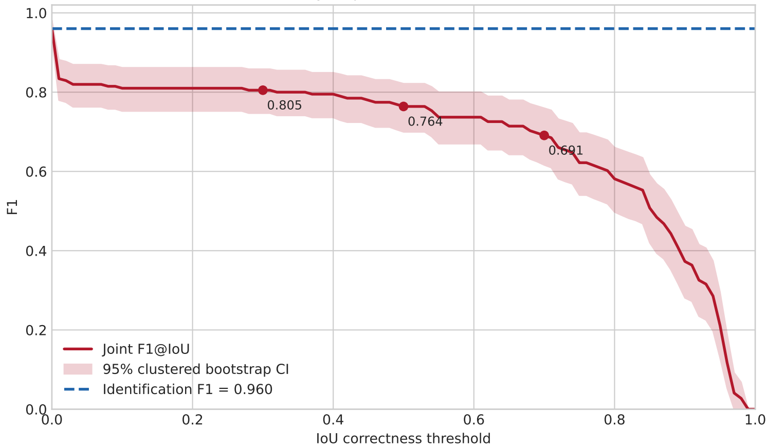
Identification-only vs joint identification-localization F1
