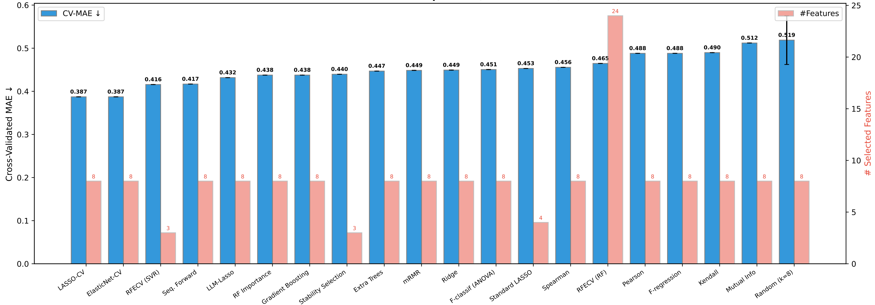
Feature Selection Method Comparison (~20 methods) — CV-MAE
