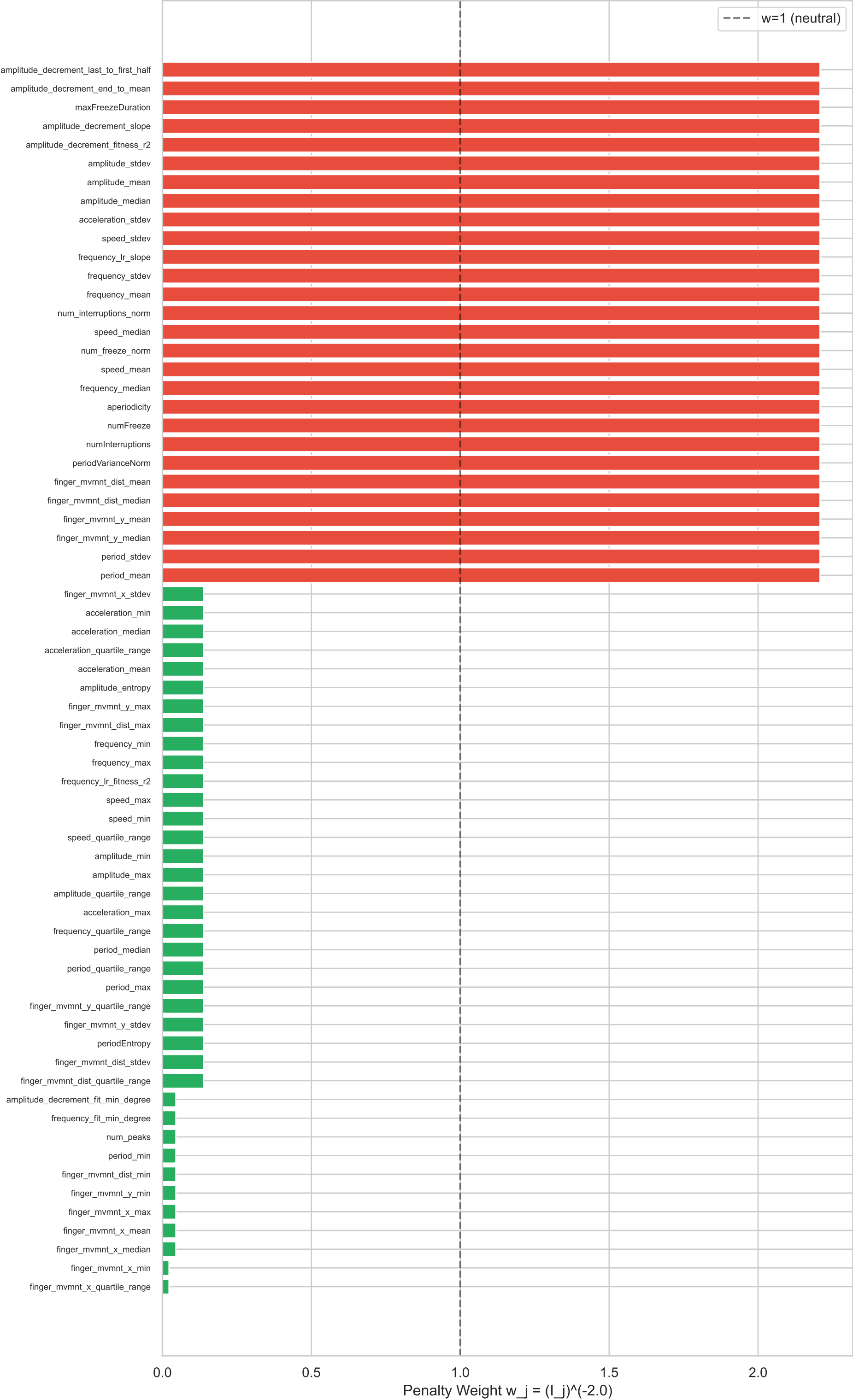
LLM-Lasso Penalty Weights ( \eta=2.0 ) Green = lower penalty (LLM says important), Red = higher penalty
