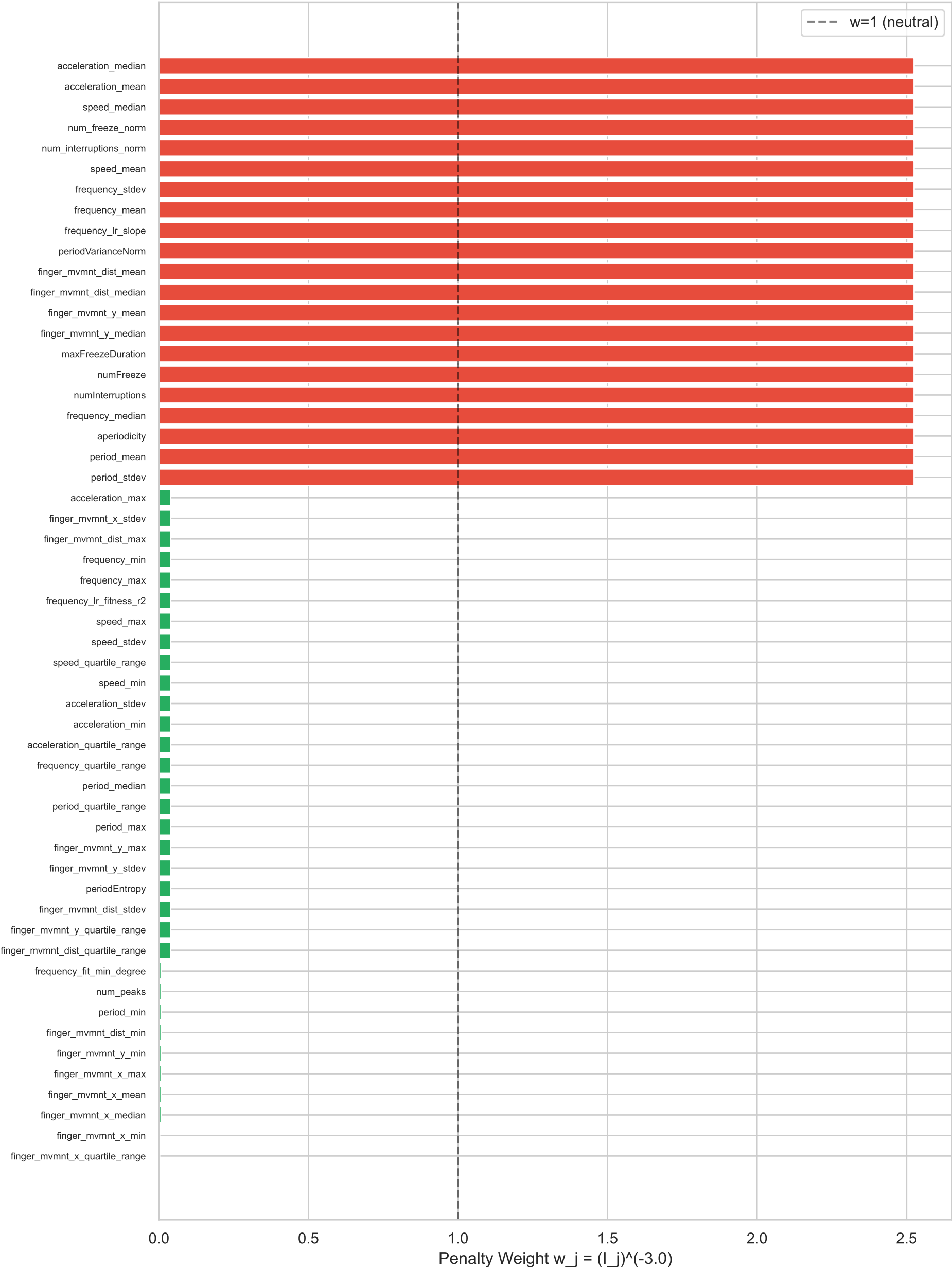
LLM-Lasso Penalty Weights ( \eta=3.0 ) Green = lower penalty (LLM says important), Red = higher penalty
