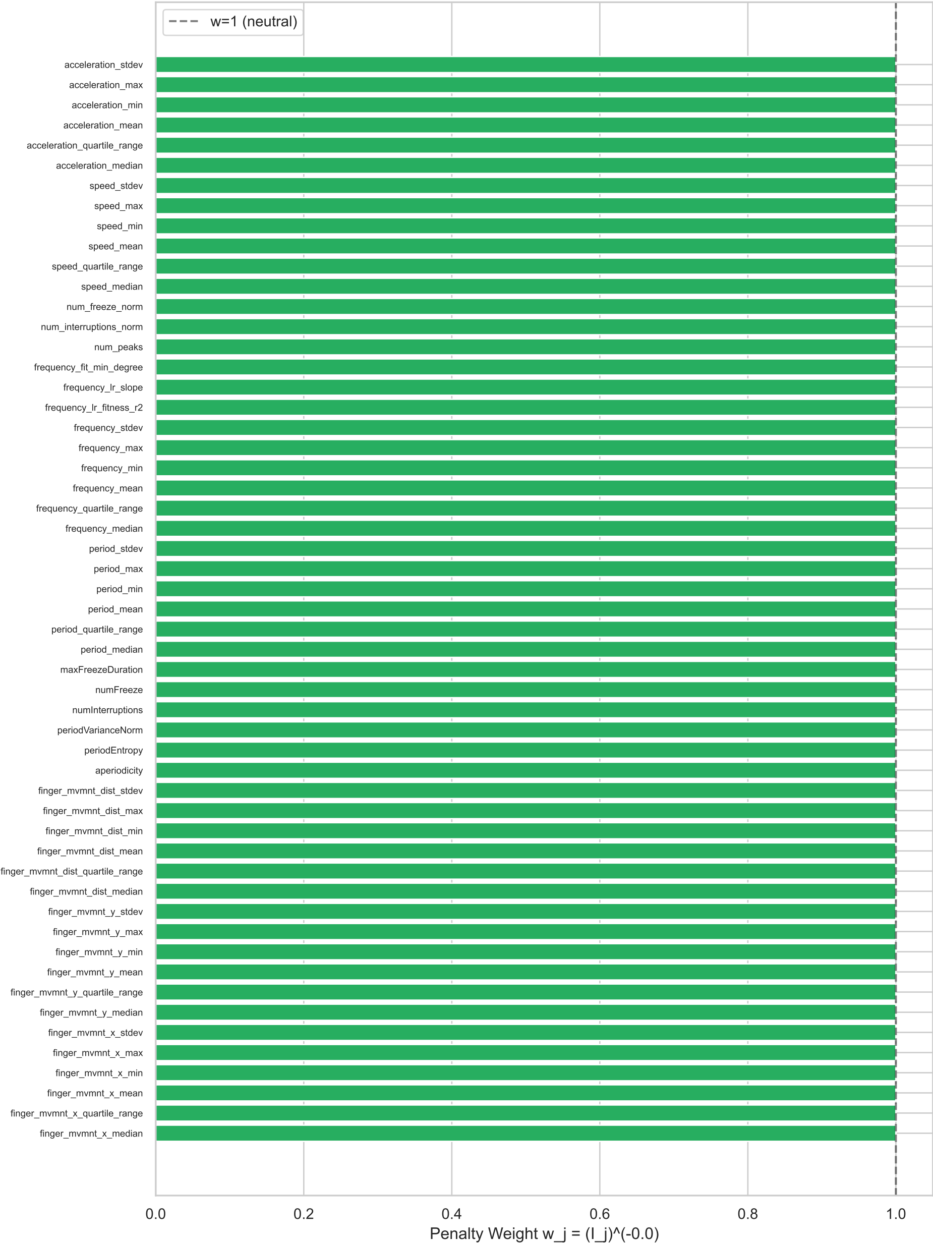
LLM-Lasso Penalty Weights ( \eta=0.0 ) Green = lower penalty (LLM says important), Red = higher penalty
