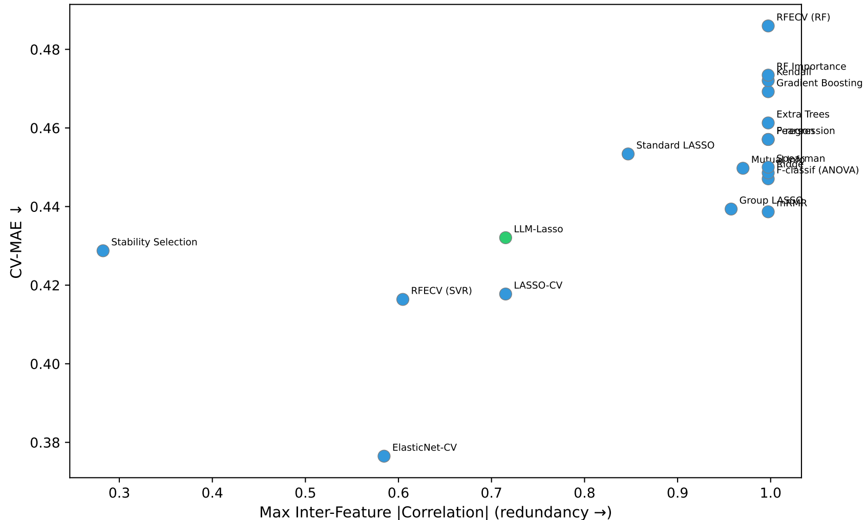
Accuracy vs Redundancy Trade-off (bottom-left = best)
