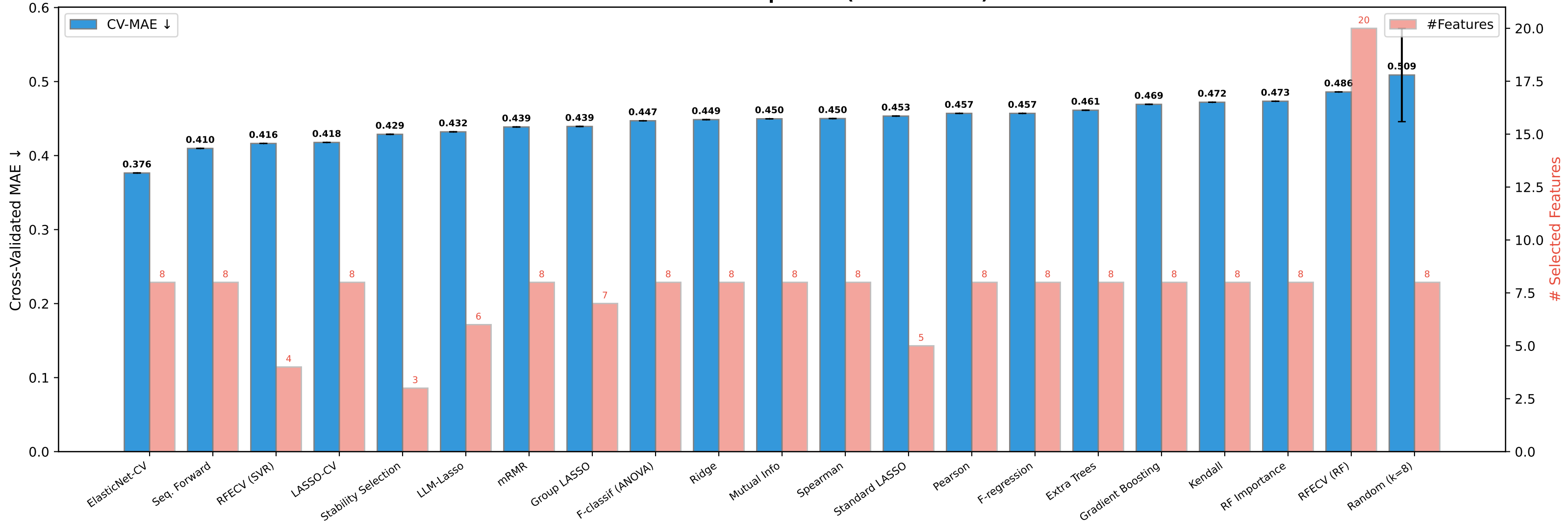
Feature Selection Method Comparison (~20 methods) — CV-MAE
