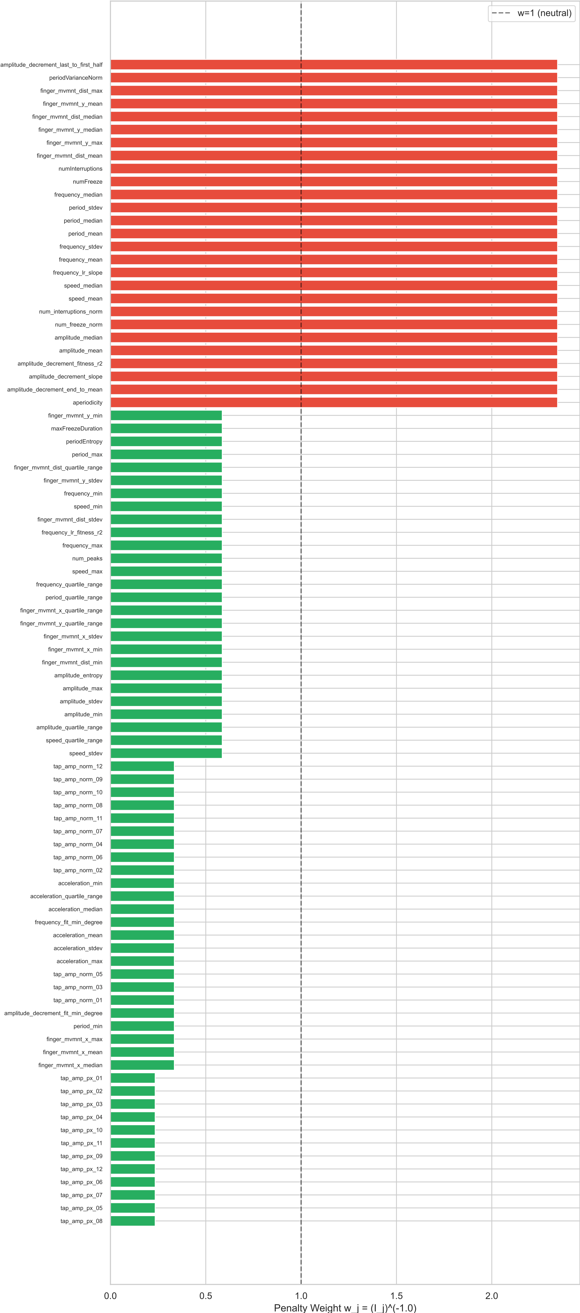
LLM-Lasso Penalty Weights ( \eta=1.0 ) Green = lower penalty (LLM says important), Red = higher penalty
