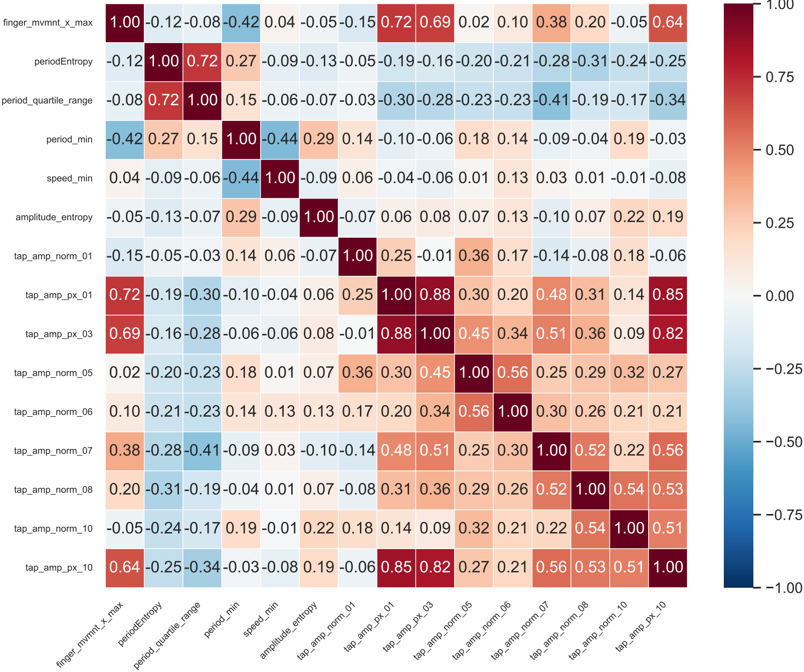
Inter-Feature Correlation Matrix (LLM-Lasso Selected)
