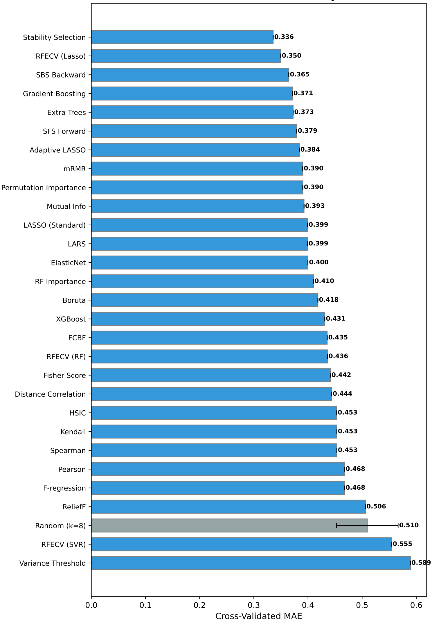
Feature Selection Methods Ranked by CV-MAE
