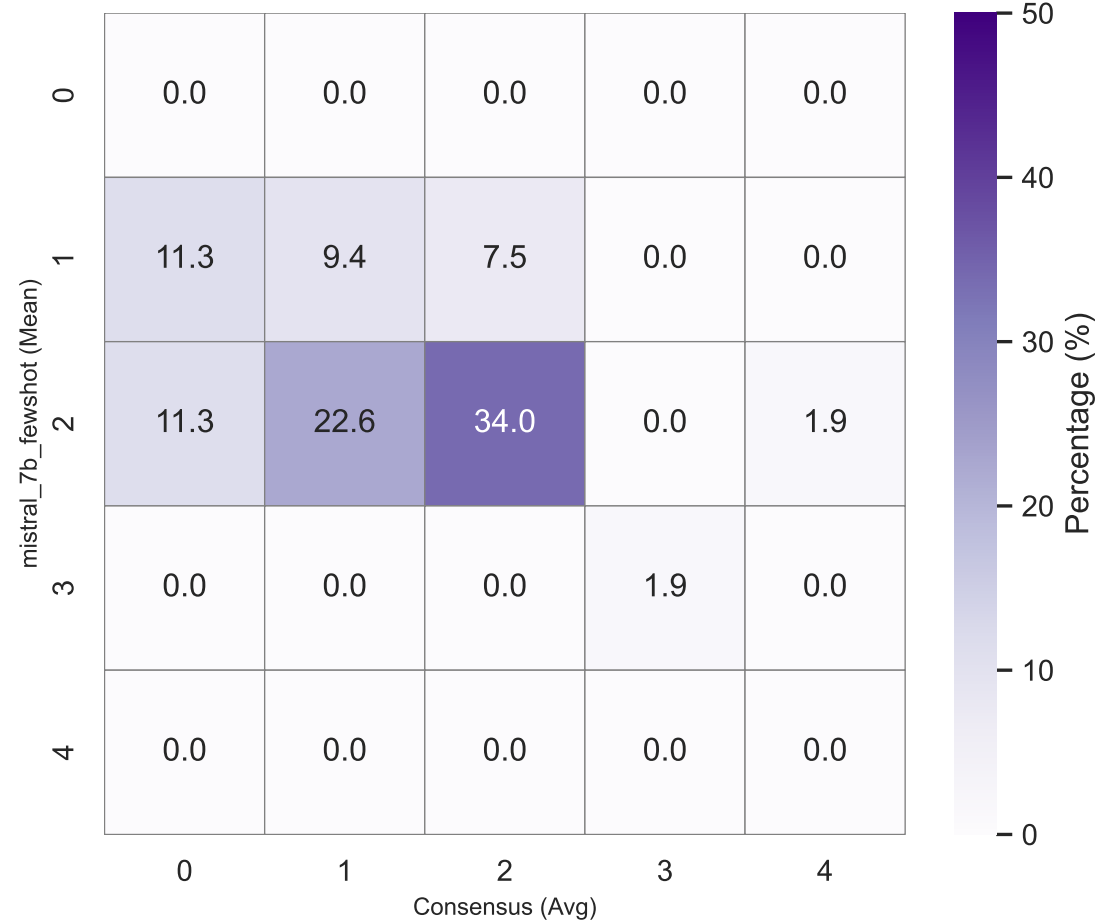
Model vs. Consensus (n=53) MAE=0.62, r=0.42, \kappa =0.24 AAUC=0.81, WD=0.43
