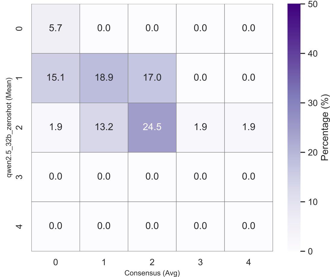
Model vs. Consensus (n=53) MAE=0.53, r=0.50, \kappa =0.46 AAUC=0.79, WD=0.29
