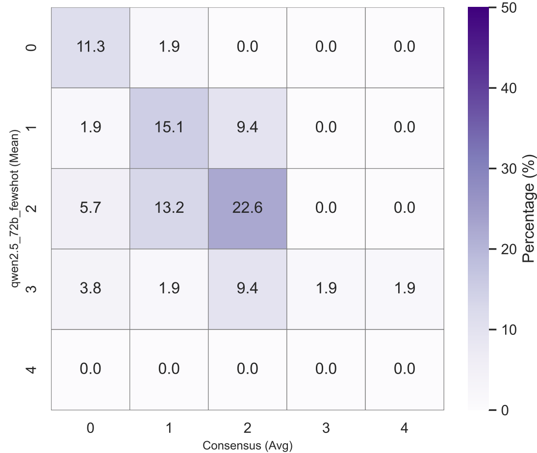
Model vs. Consensus (n=53) MAE=0.61, r=0.49, \kappa =0.44 AAUC=0.71, WD=0.37
