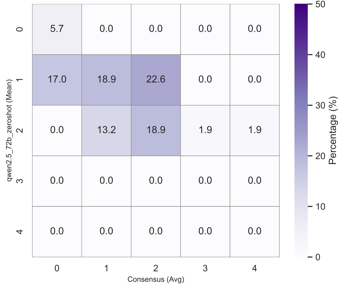
Model vs. Consensus (n=53) MAE=0.54, r=0.53, \kappa =0.45 AAUC=0.77, WD=0.26
