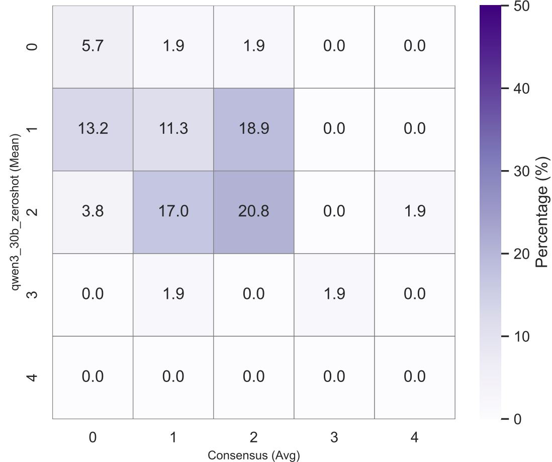
Model vs. Consensus (n=53) MAE=0.67, r=0.33, \kappa =0.33 AAUC=0.67, WD=0.18
