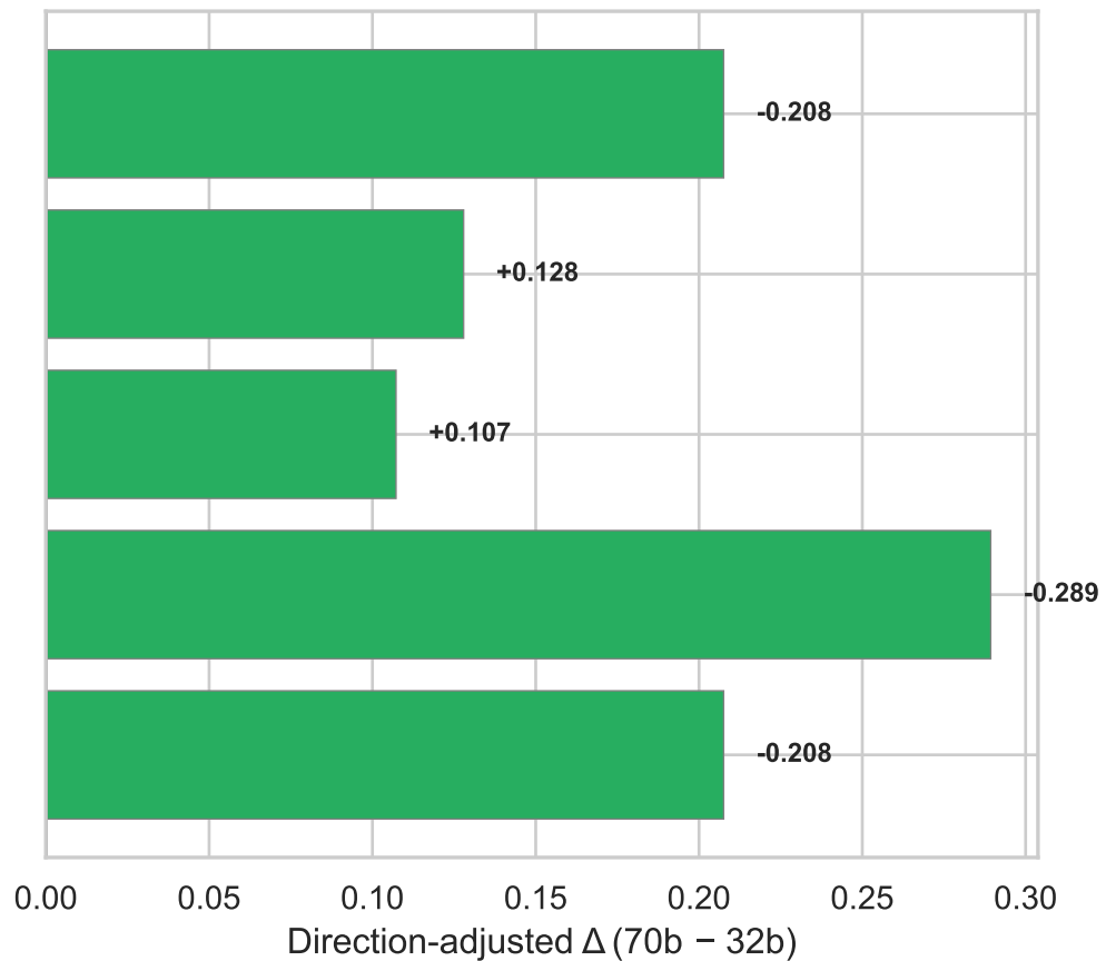
Zeroshot
