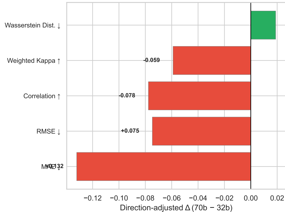
Fewshot
