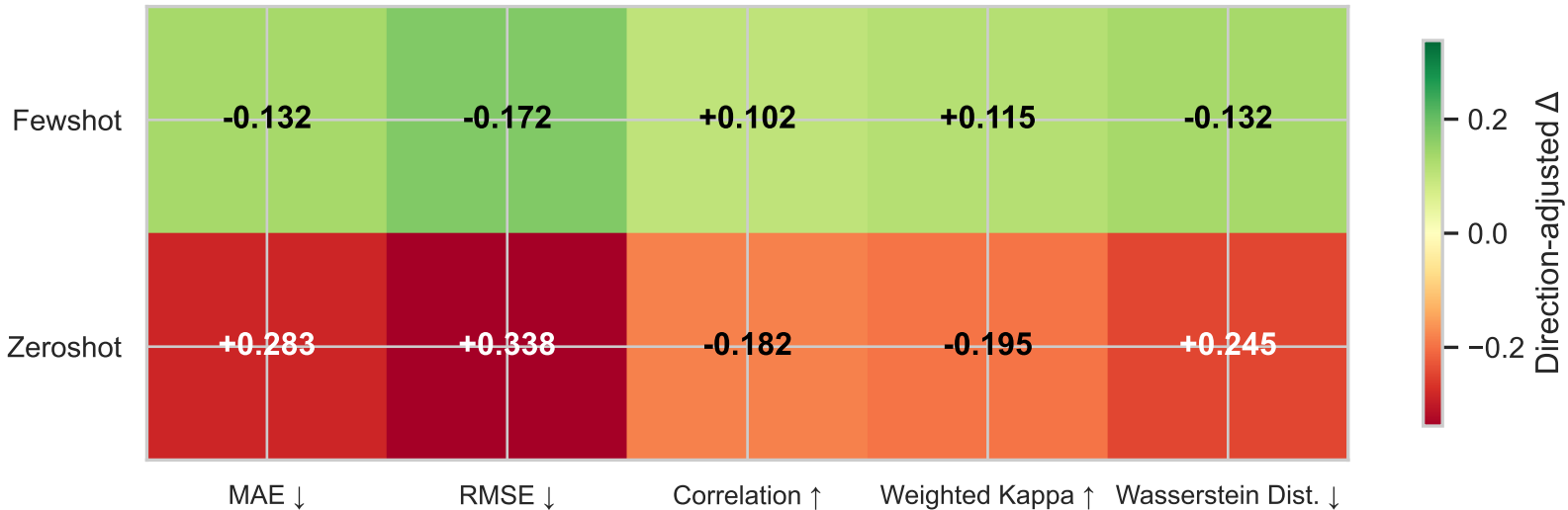
\Delta (DeepSeek-R1-32b – Qwen2.5-32b): direction-adjusted Green = Reasoning distillation helps | Red = Base model better
