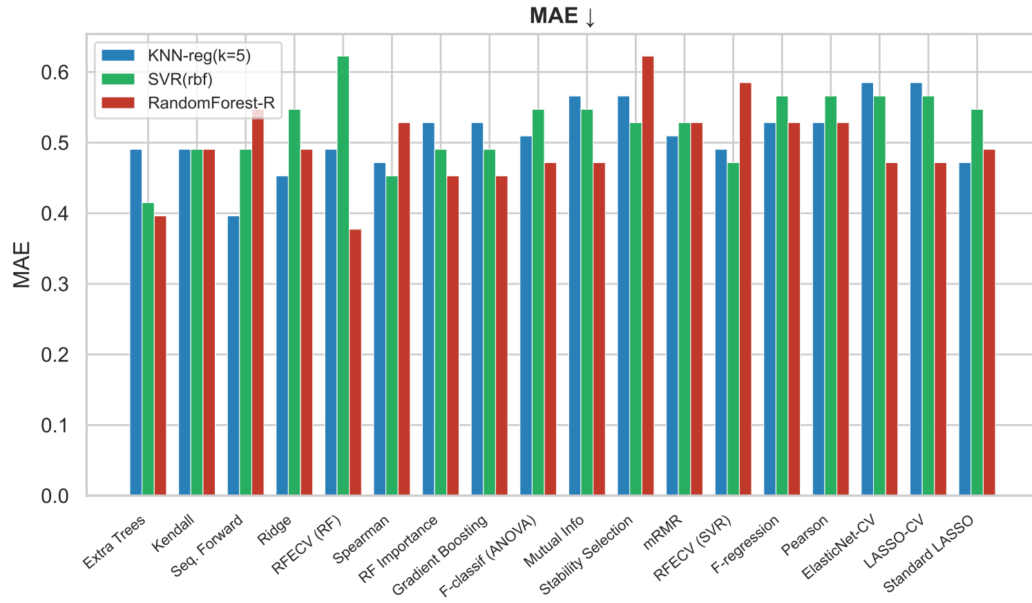
Feature Selection Methods – Per-Metric Comparison (grouped bars = KNN / SVR / RF; ordered by mean composite)
