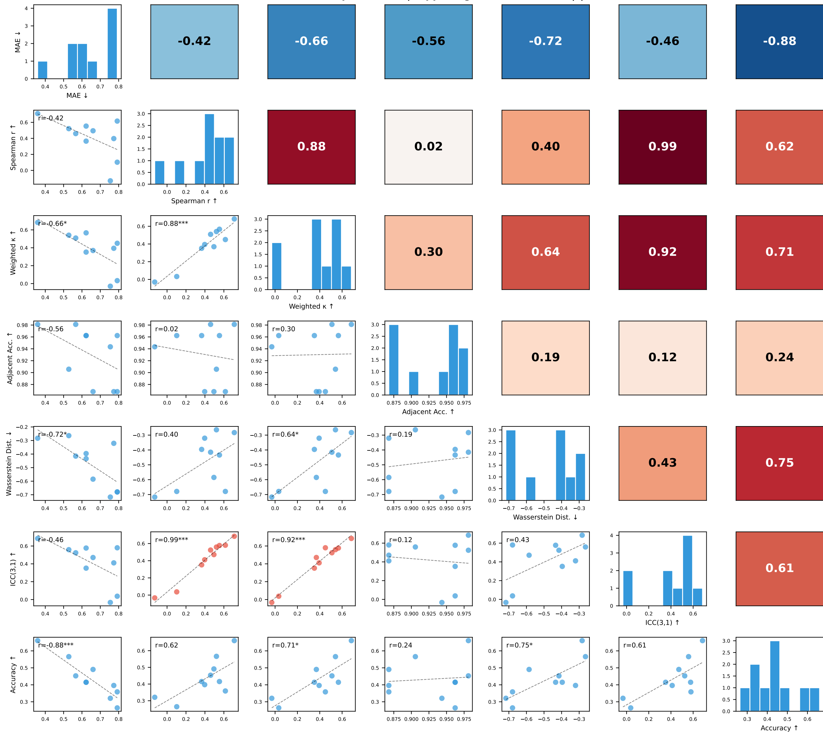
Metric Scatter Matrix (LLM experiments, n=10) Lower-left: scatter + Spearman r | Upper-right: r value (red = |r| > 0.9 )
