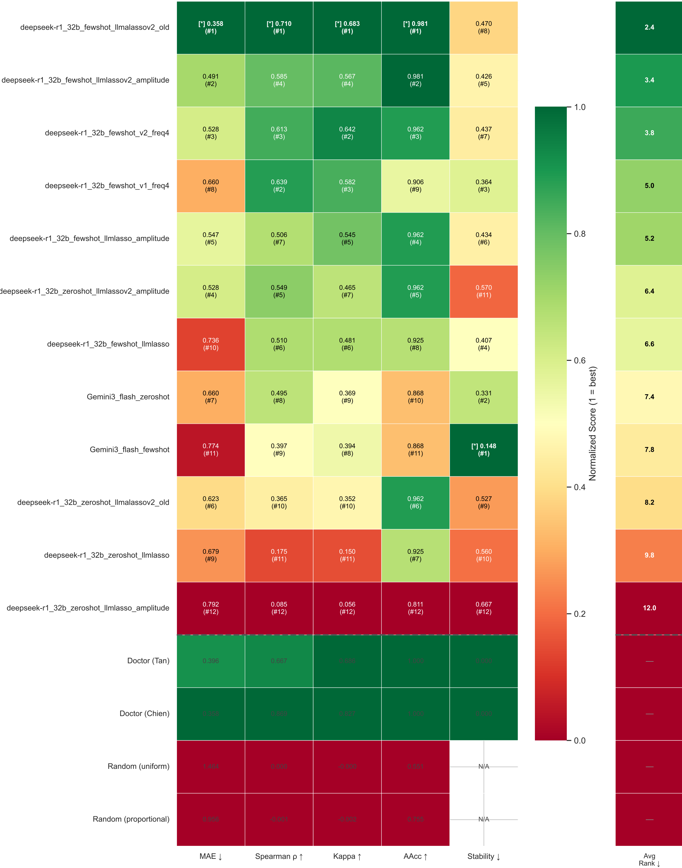
Model Performance Heatmap (green = better, [*] = best per metric)
