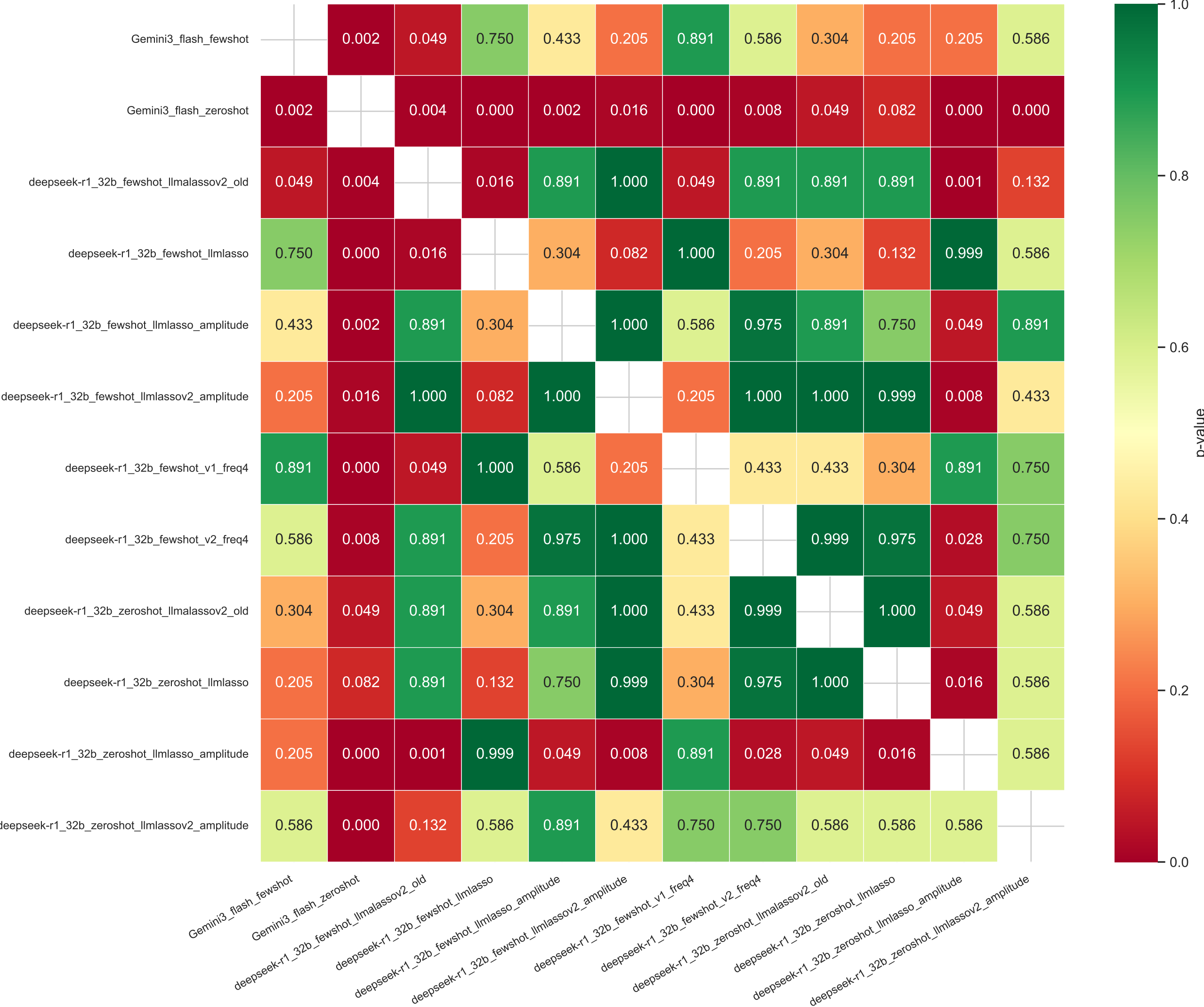
Pairwise KS Test p-values (error distribution comparison)
