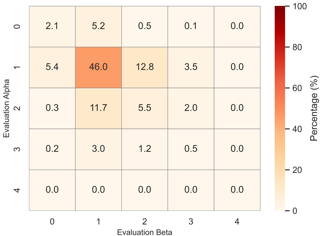
Model Consistency (scored_by_ChatGPT_prompt3)
