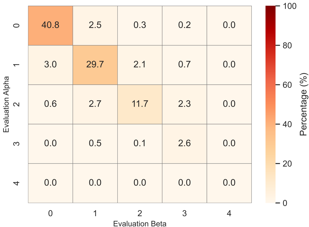
Model Consistency (scored_by_Gemini3pro_promptC_10)
