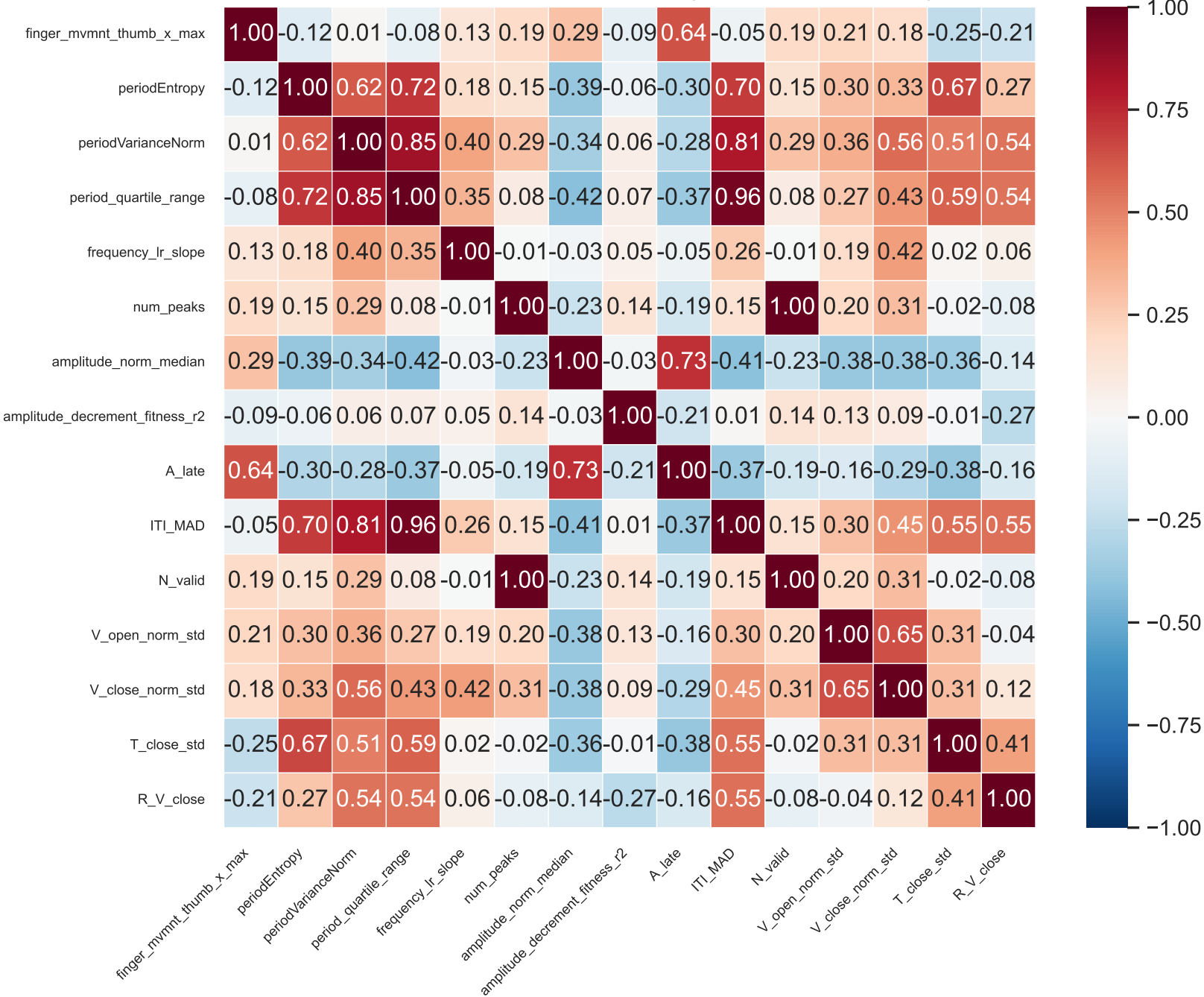
Inter-Feature Correlation Matrix (LLM-Lasso Selected)
