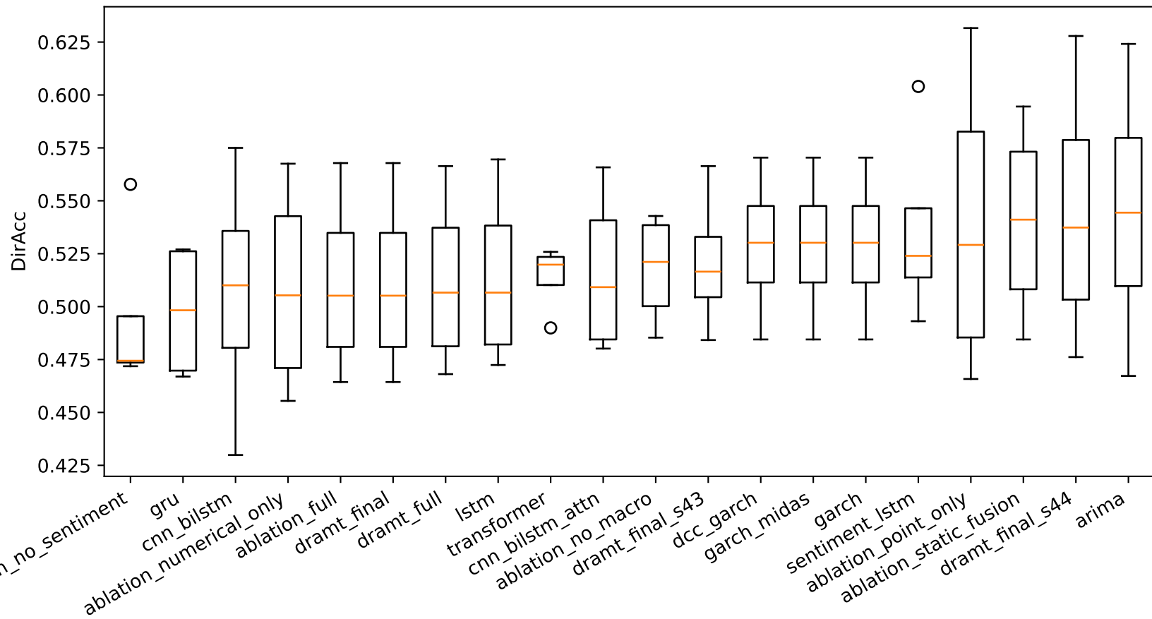
Per-fold DirAcc across models
