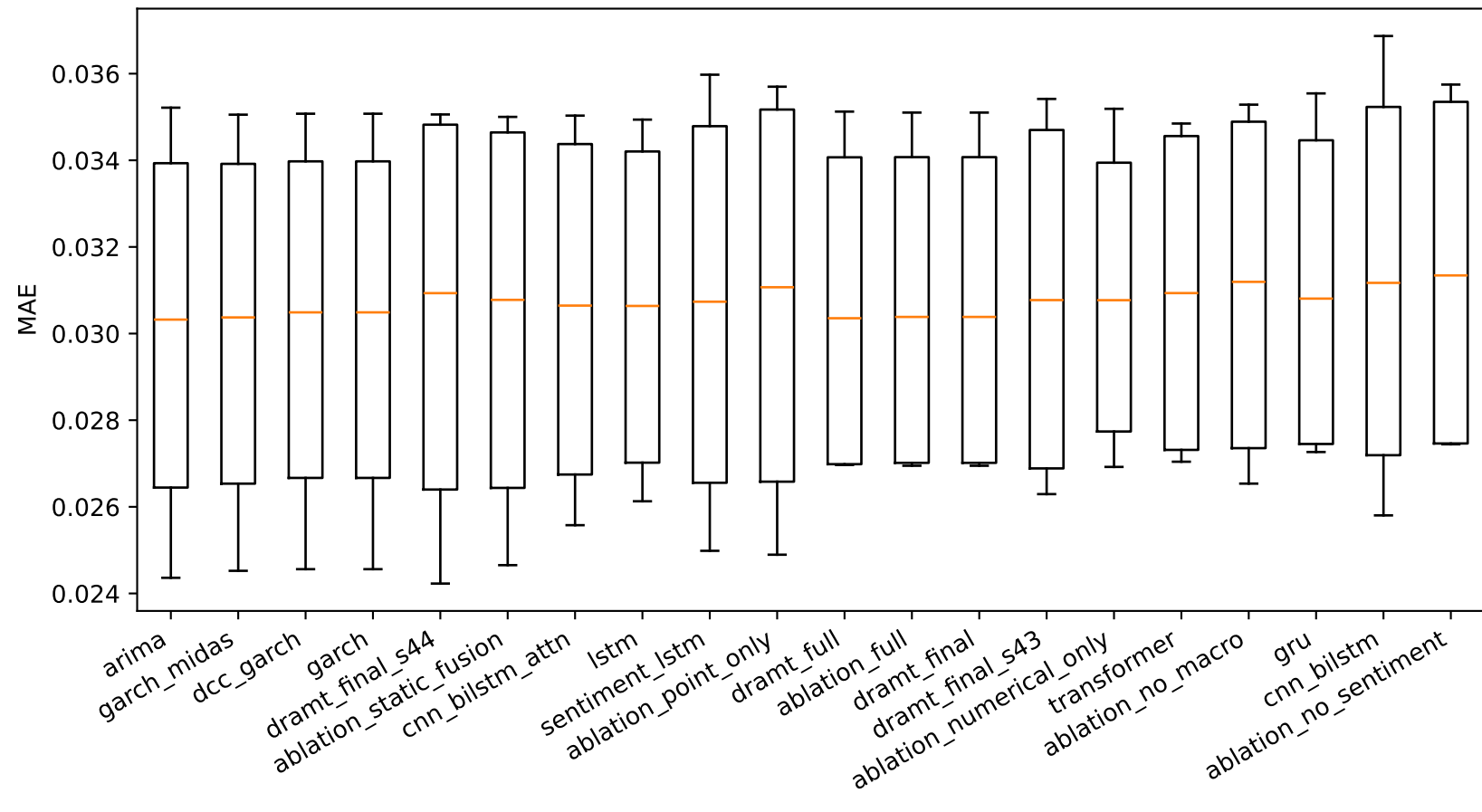
Per-fold MAE across models
