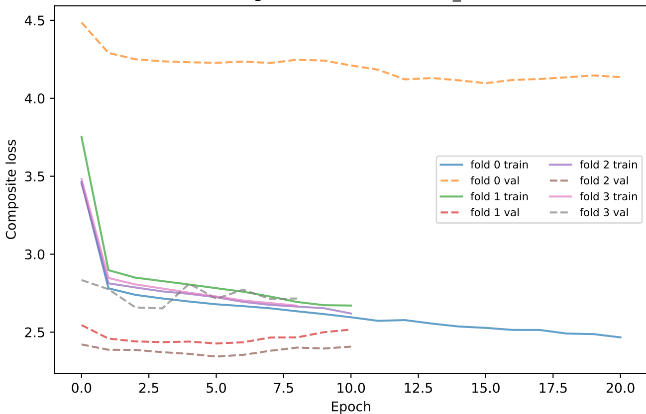
Training / validation loss (dramt_final)
