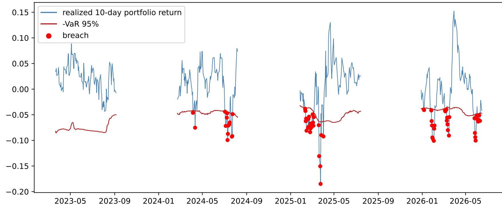
Portfolio 10-day VaR backtest (all test folds)
