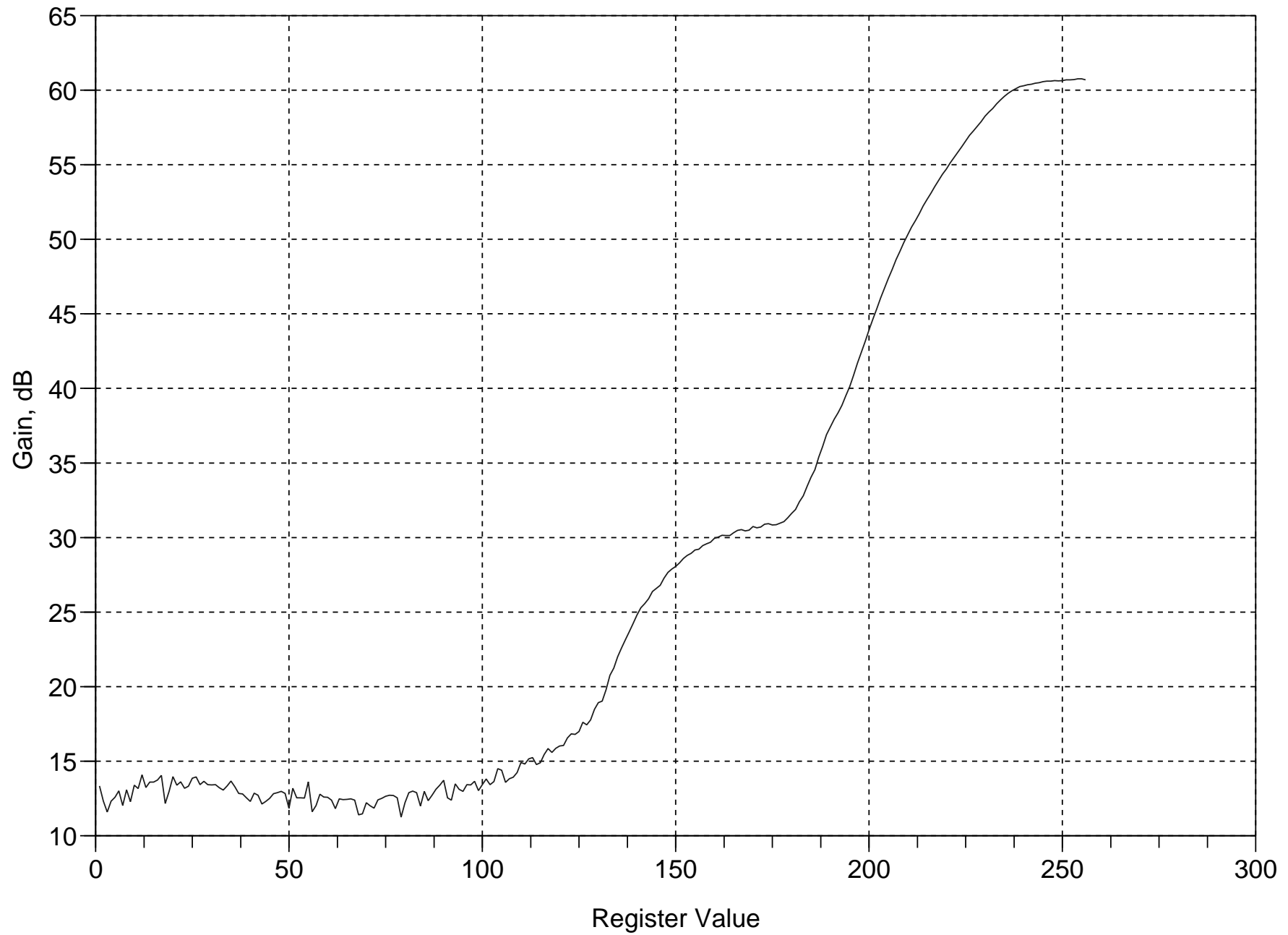
R82xx Tuner Gain vs. RTL2832U AGC Register Setting
