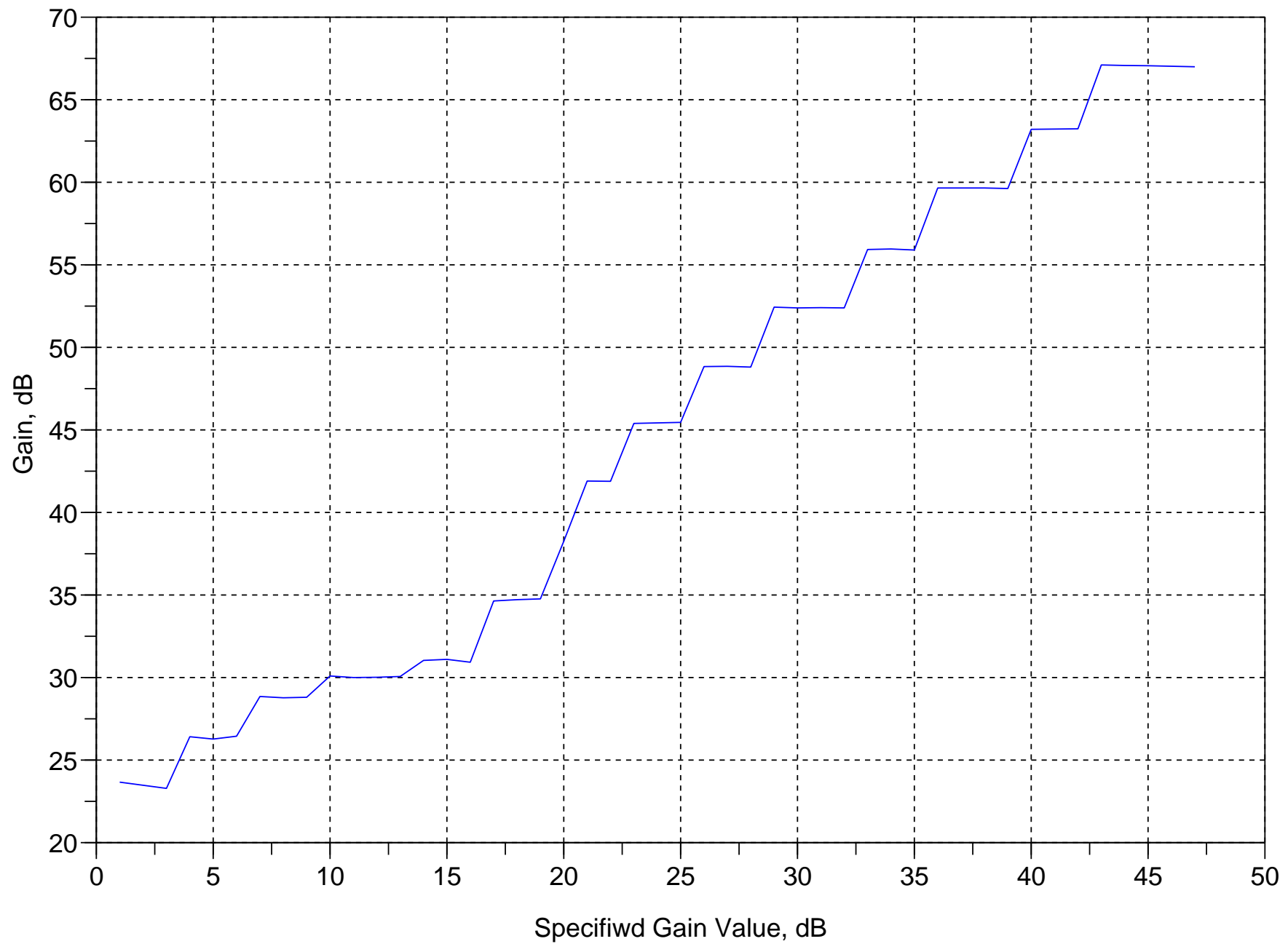
R82xx Tuner Gain vs. R82xx AGC Register Setting
