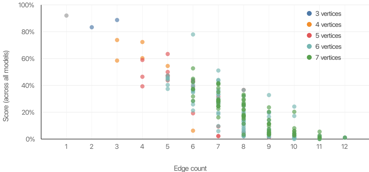
Task Score vs Edge Count ( r = -0.85 )
