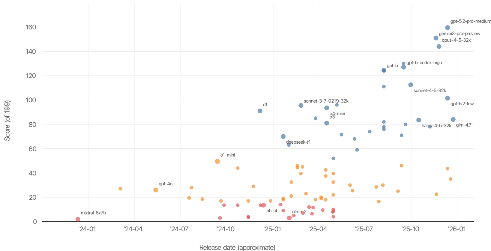
Benchmark Score vs Model Release Date
