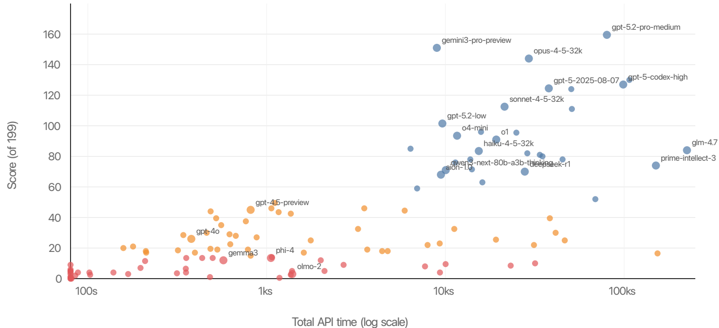
Benchmark Score vs Total API Time
