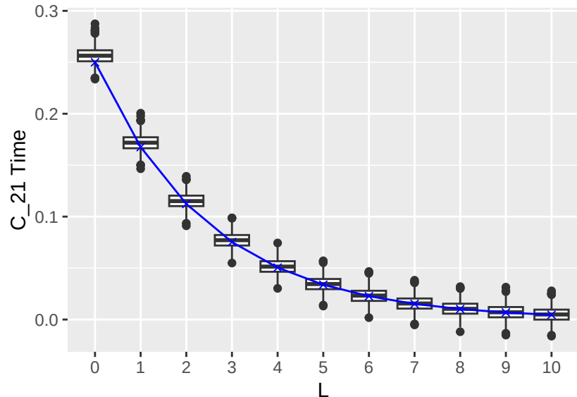
C_{21}^T(L) boxplots over 1000 realisations of field
