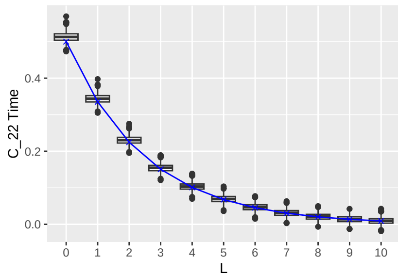
C_{22}^T(L) boxplots over 1000 realisations of field
