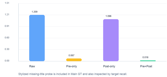
Pre/Post Ablation (main GT, N=784)
