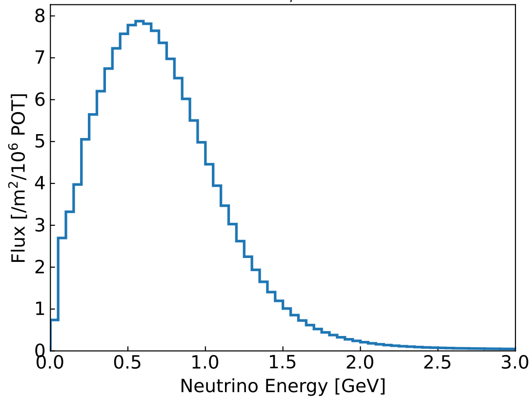
SBND \nu_\mu Flux
