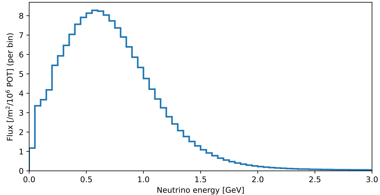
SBND \nu_\mu flux — nominal
