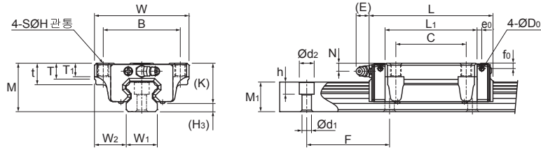
HSR15~65C/LC/XC/XLC
