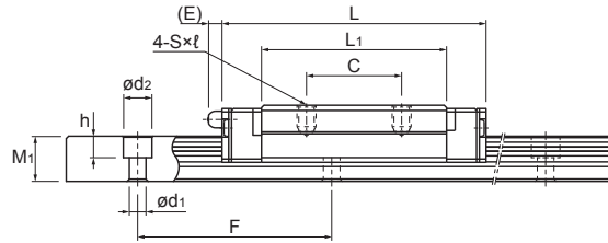
RSX 15, 15N
