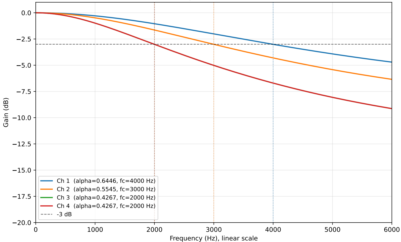
Corrected per-channel alpha values, fs=22000 Hz (retuned to actually hit 4kHz / 3kHz / 2kHz / 2kHz)
