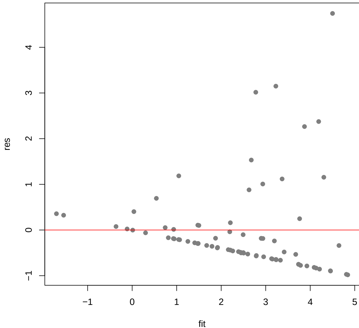
Residuals vs Fitted ( Wildfire OLS )
