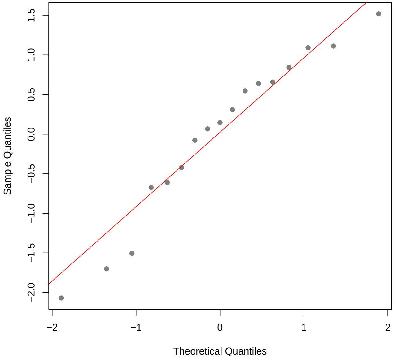
QQ Plot ( California )
