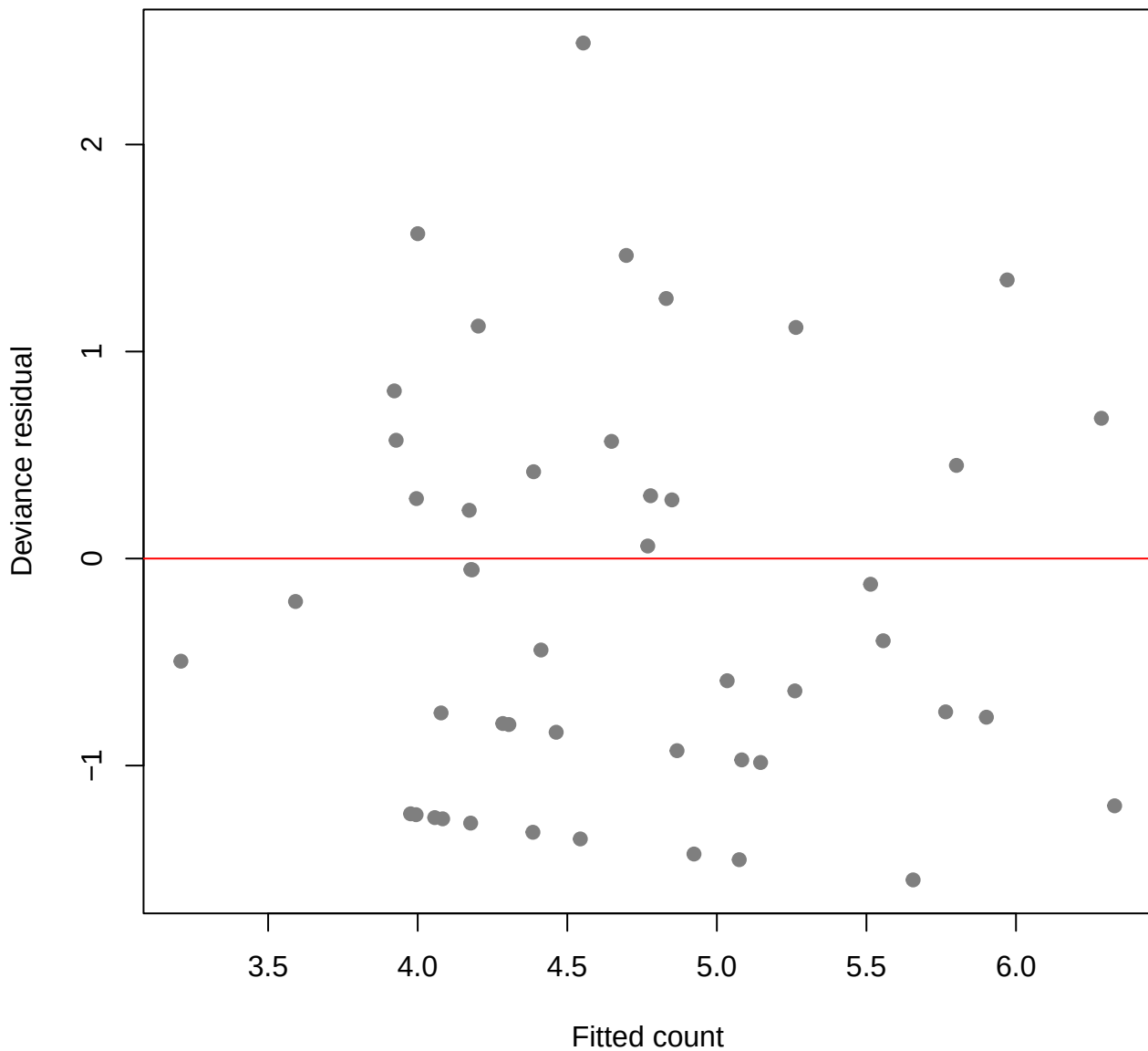
Deviance Residuals vs Fitted (Negative Binomial, SC)
