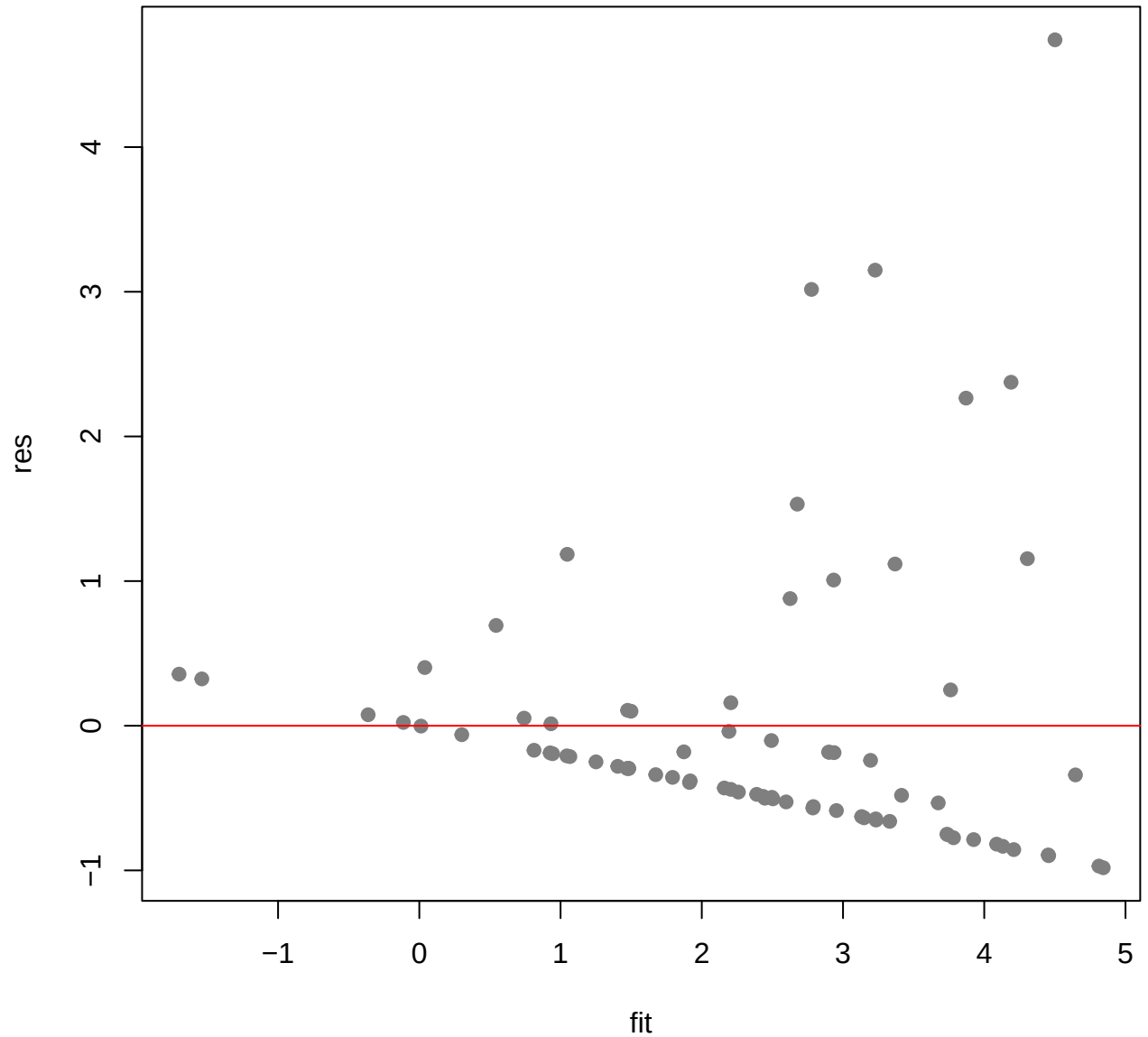
Residuals vs Fitted ( Wildfire OLS )
