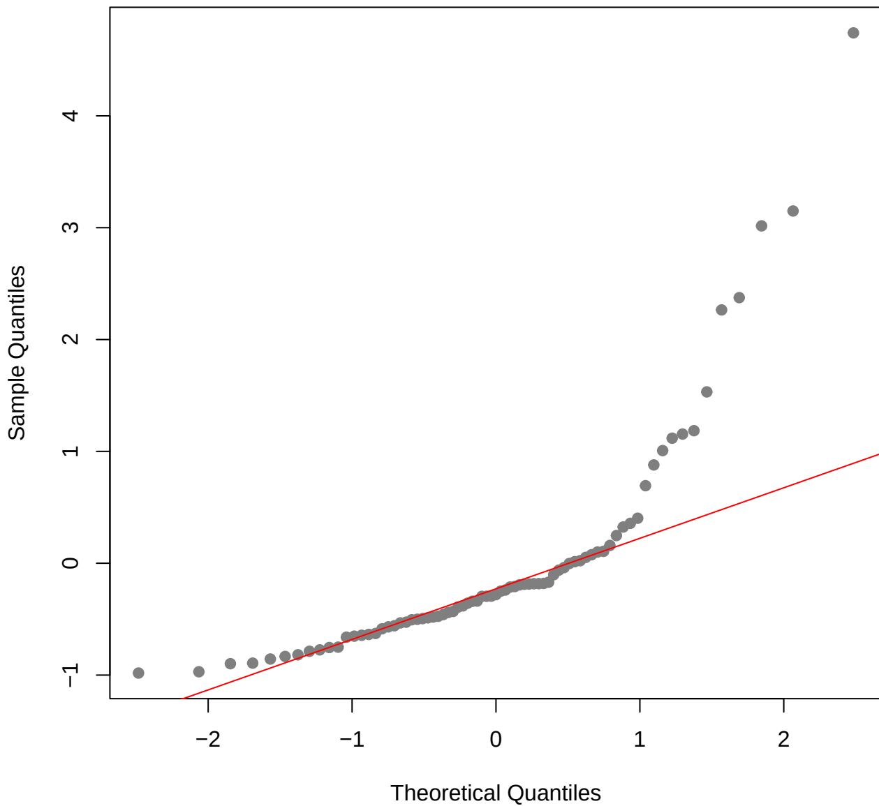
QQ Plot ( Wildfire OLS )
