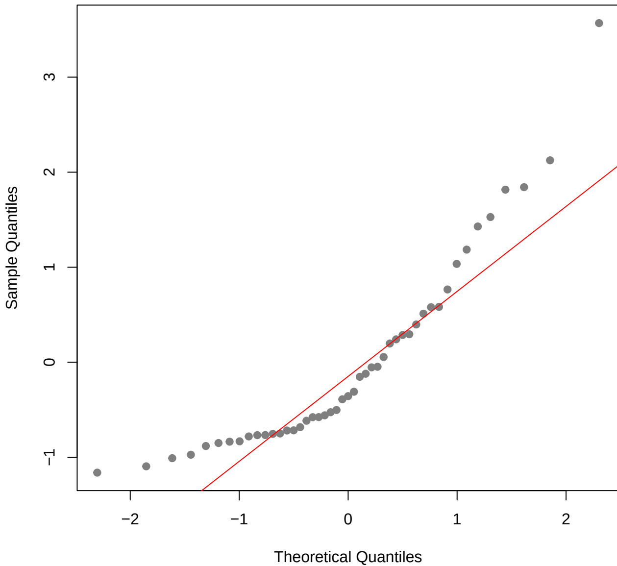
QQ Plot ( South Carolina, logged )
