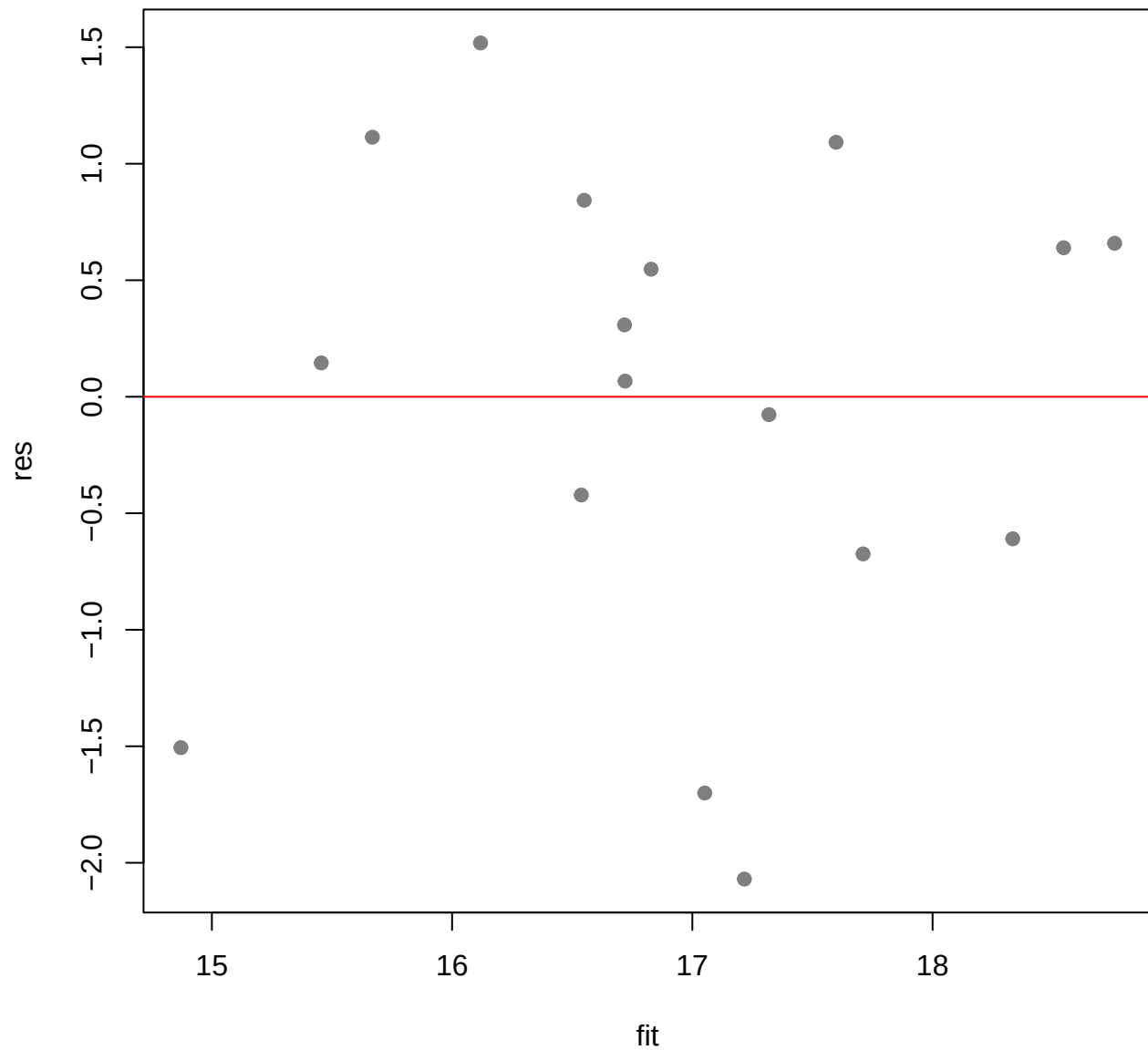
Residuals vs Fitted ( California )
