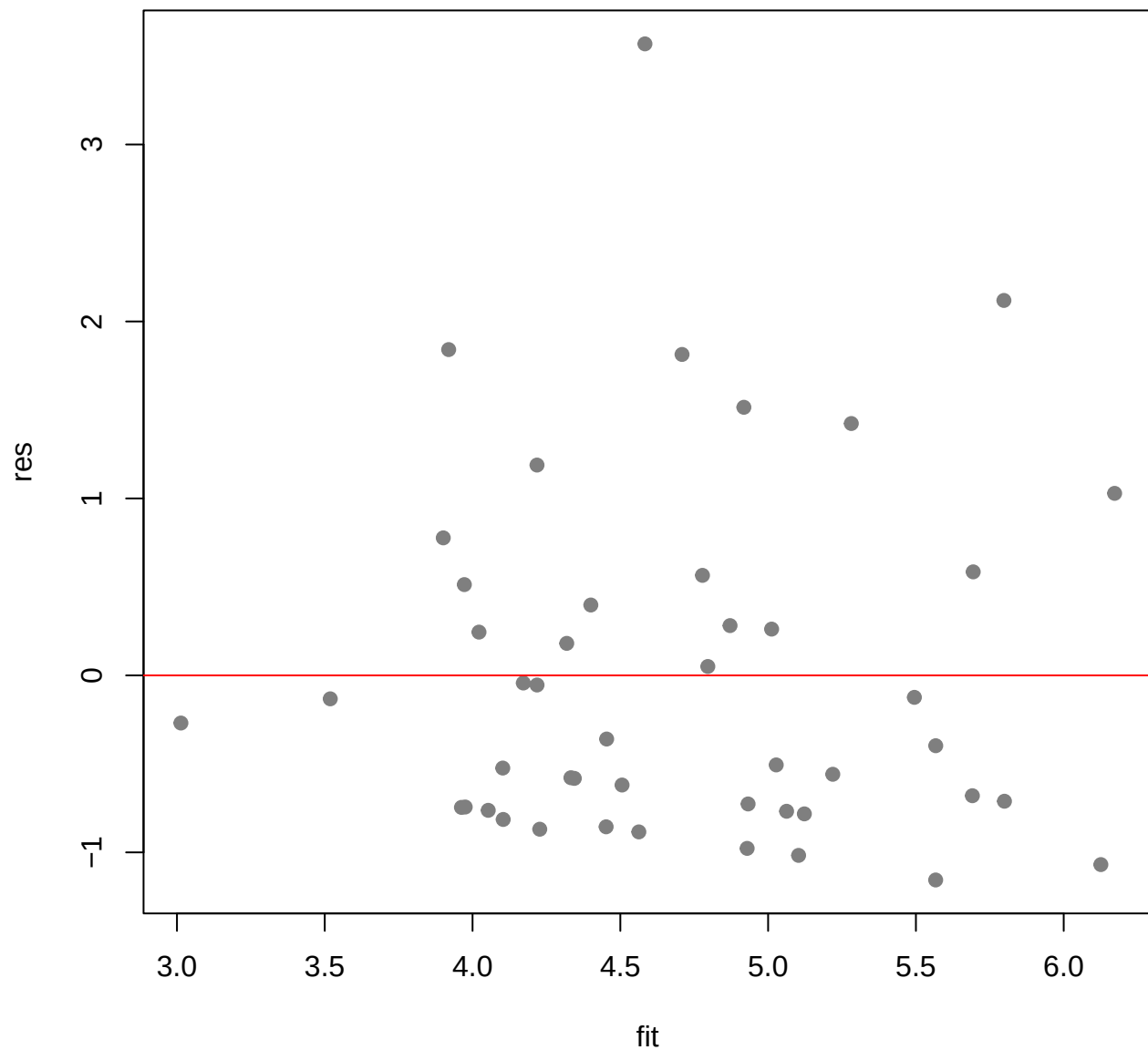
Residuals vs Fitted ( South Carolina )
