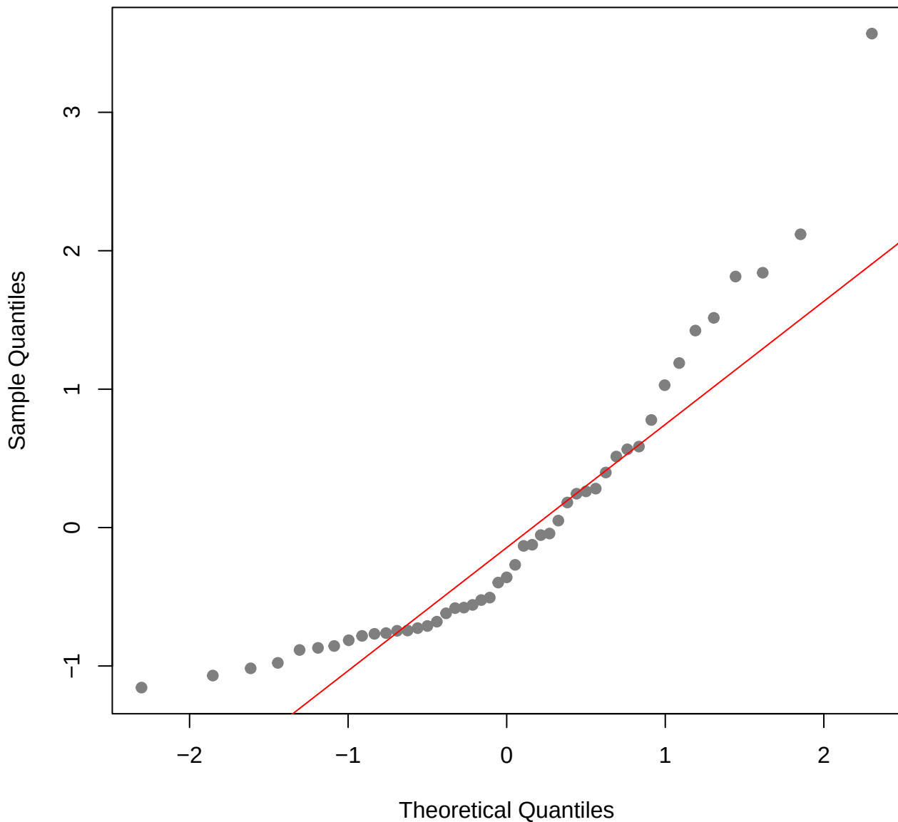
QQ Plot ( South Carolina )
