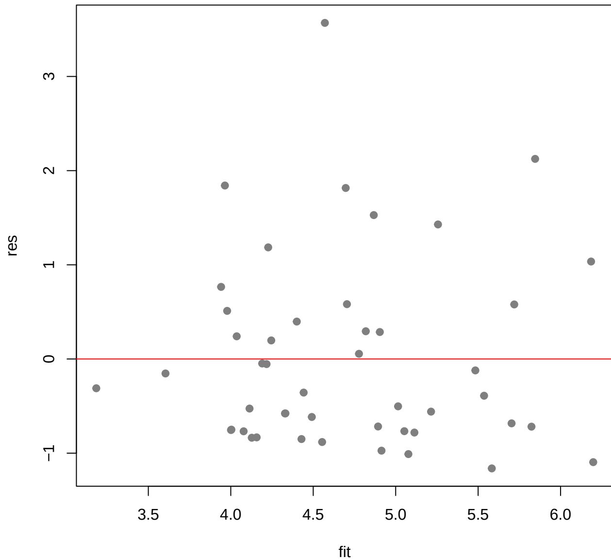
Residuals vs Fitted ( South Carolina, logged )
