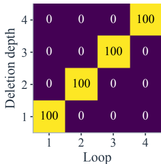
(a) Stepwise
