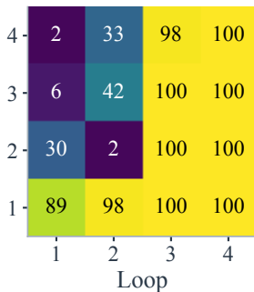
(b) Final-only
